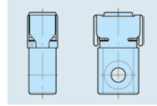
Matrize / die 951.XX (R-DF 6) a_{ges} = \max. 3.0 \text{ mm}
