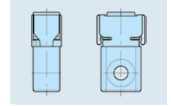
Matrize / die 950.XX (R-DF 8) a_{ges} = \max. 3.0 \text{ mm}
